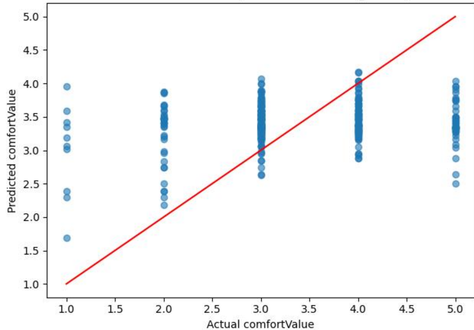
Predicted vs Actual (Random Forest Regressor)
